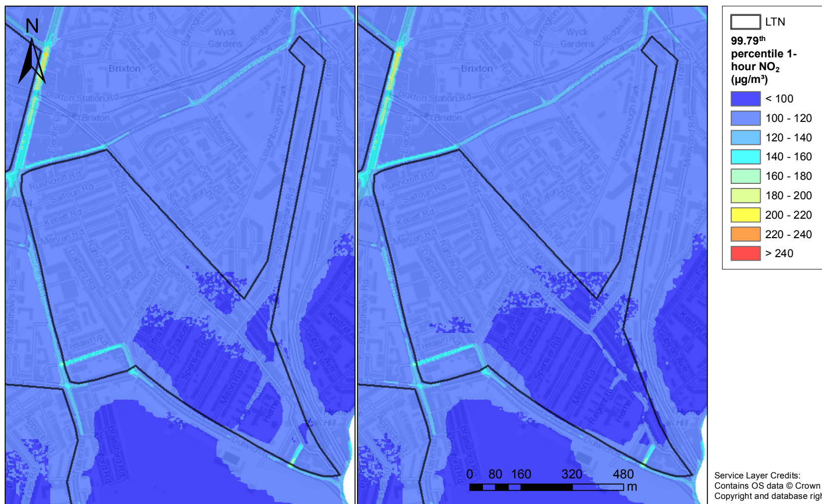
Figure 6.5: Pre-Scheme (left) and Post-Scheme (right) 99.79 th percentile of hourly average NO 2 concentrations (µg/m 3 ), Railton LTN
