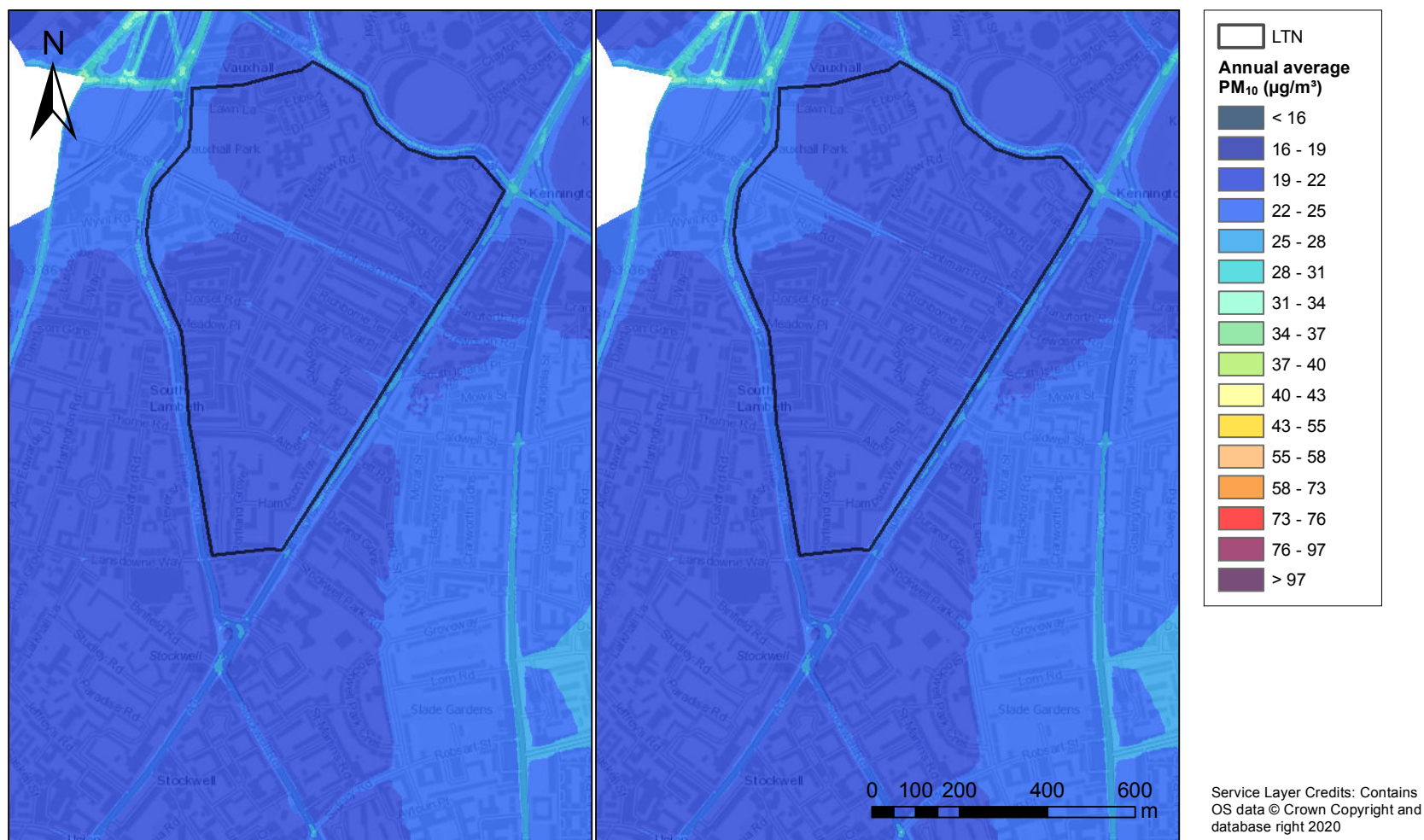
Figure 6.6: Pre-Scheme (left) and Post-Scheme (right) annual average PM_{10} concentrations ( \mu g/m^3 ), Oval LTN
