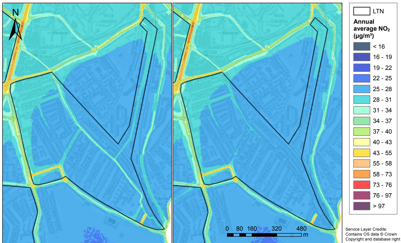
Figure 6.3: Pre-Scheme (left) and Post-Scheme (right) annual average \text{NO}_2 concentrations ( \mu\text{g}/\text{m}^3 ), Railton LTN
