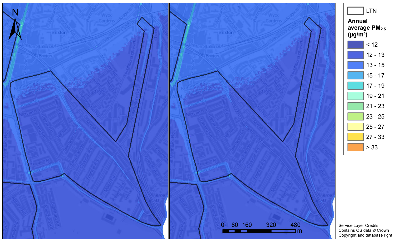
Figure 6.11: Pre-Scheme (left) and Post-Scheme (right) annual average PM_{2.5} concentrations ( \mu g/m^3 ), Railton LTN
